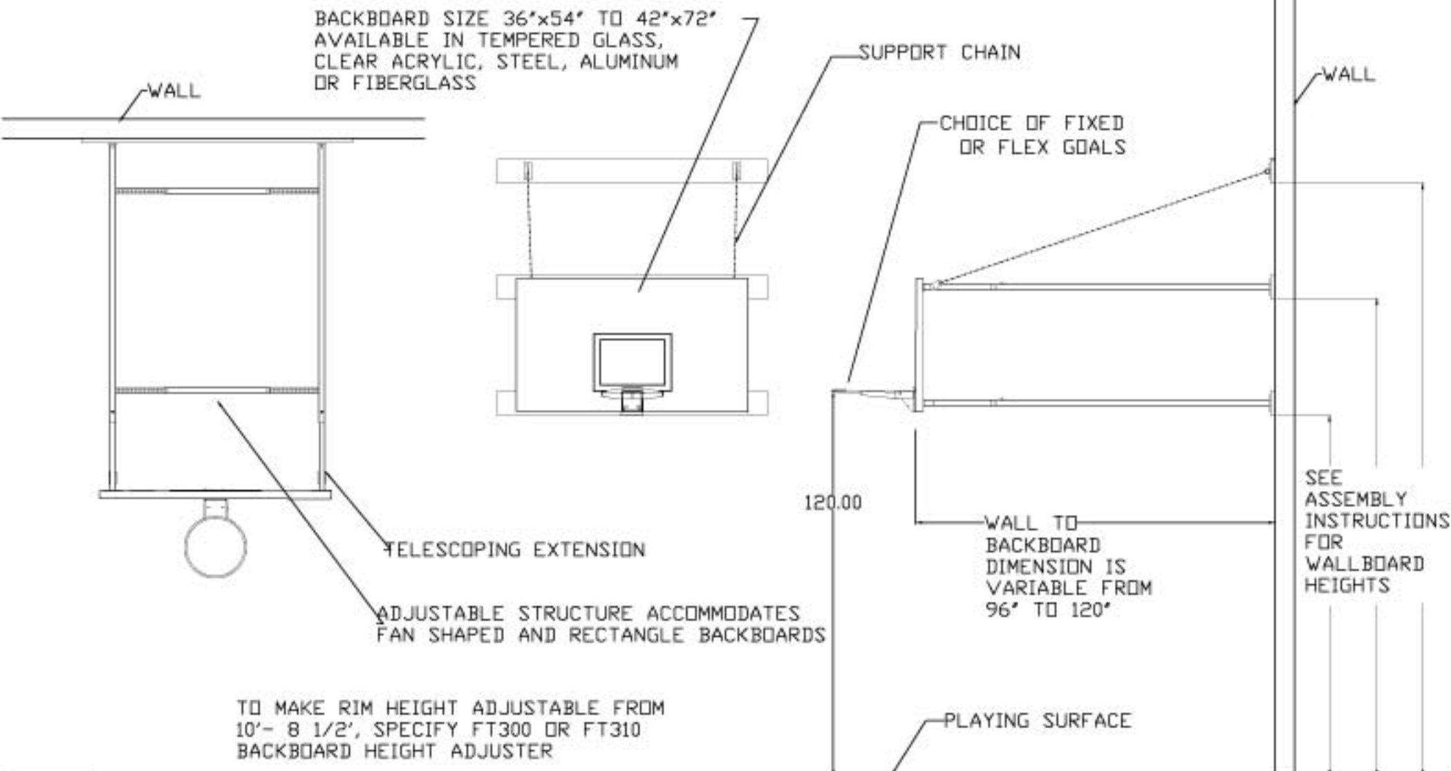
FRONT VIEW
