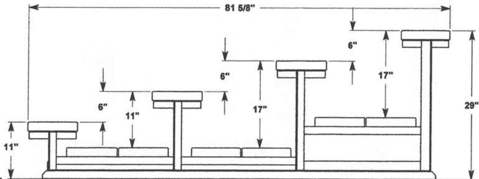
FANSTAND 4 Row w/double footplank
