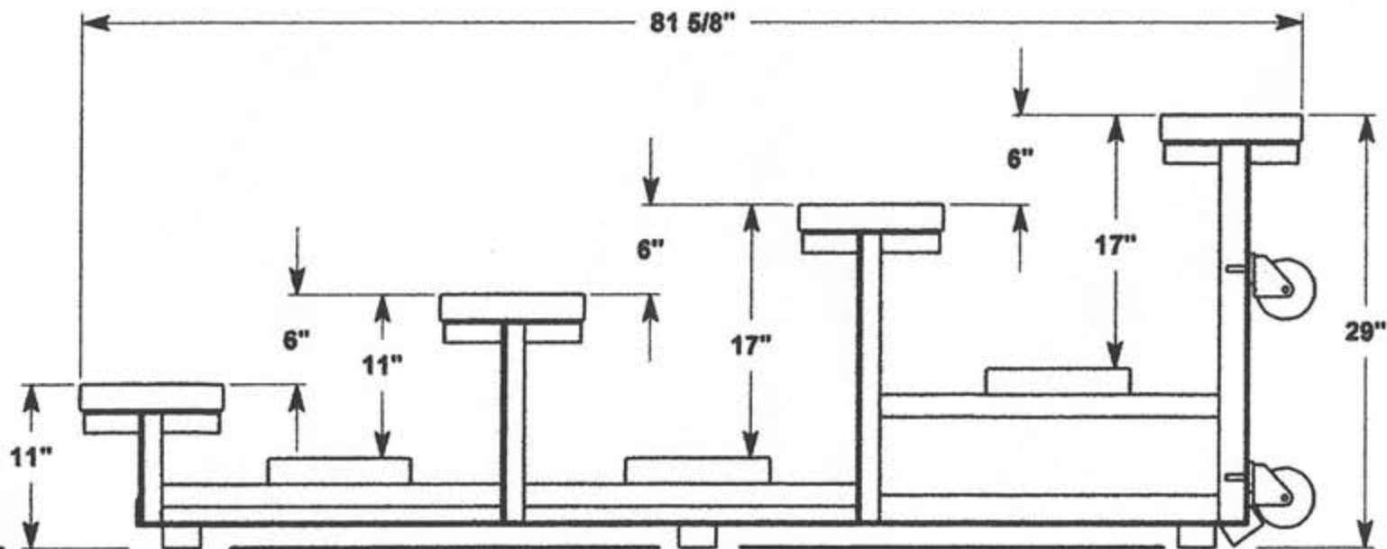
FANSTAND 4 Row w/single footplank Tip N Roll Bleacher
