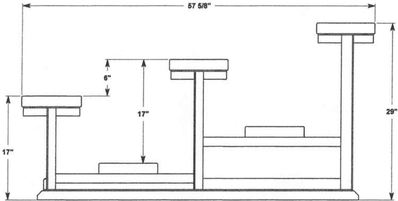
FANSTAND 3 Row w/single footplank
