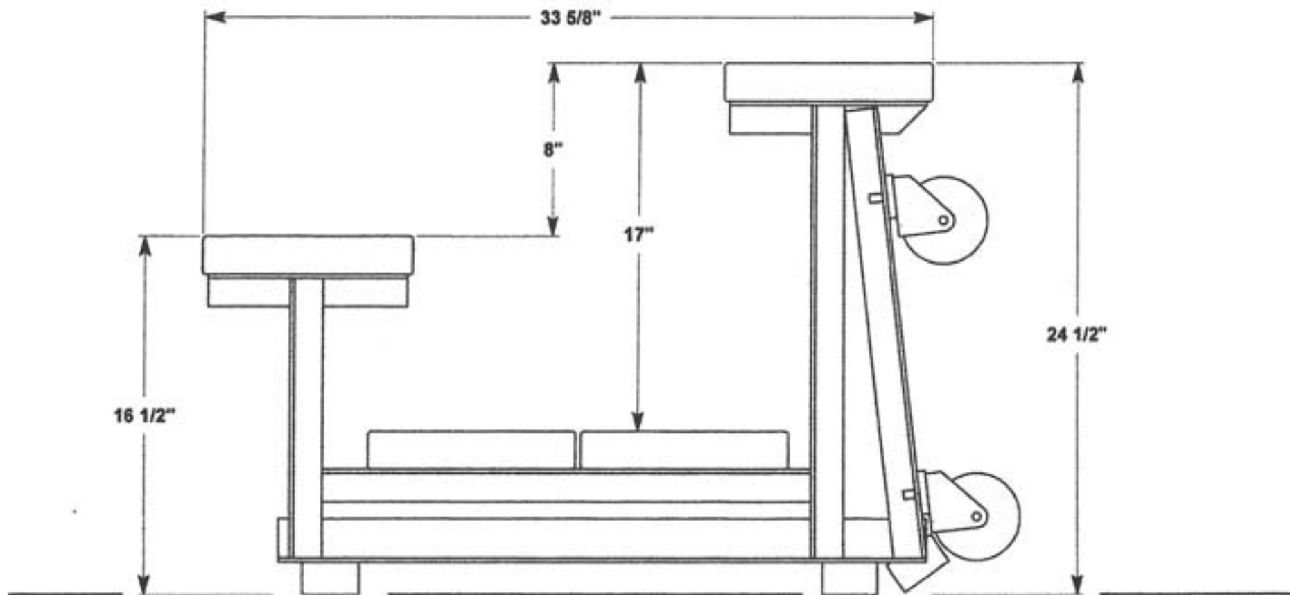
FANSTAND 2 Row w/double footplank Tip N Roll Bleacher
