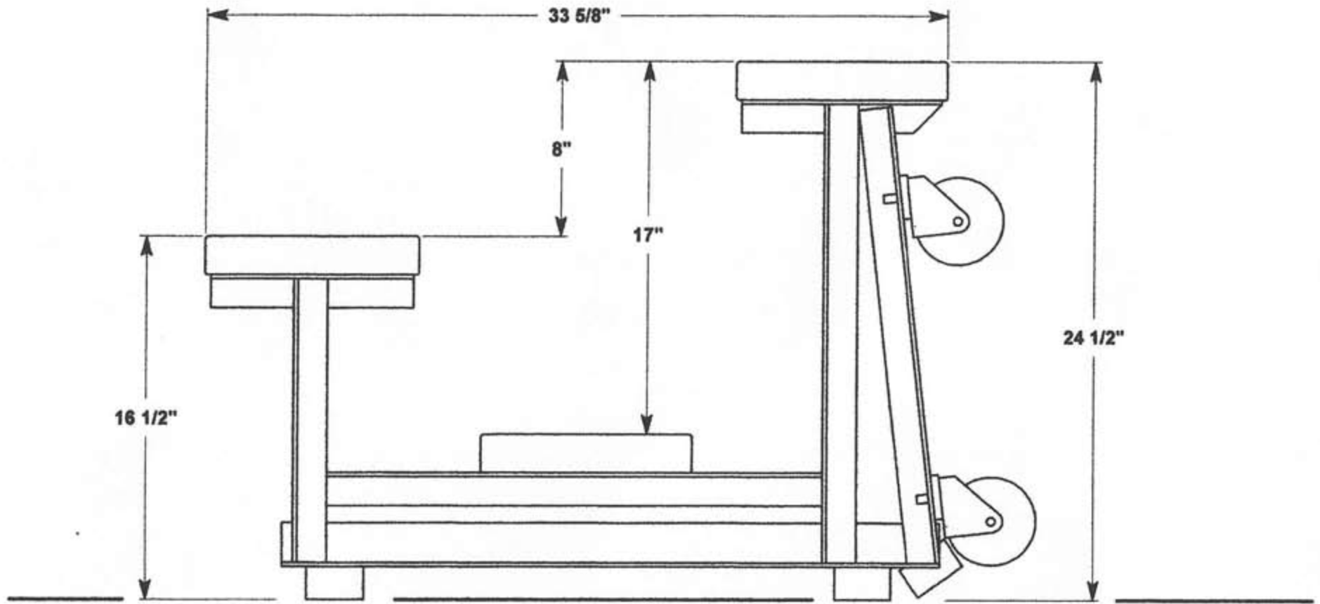
FANSTAND 2 Row w/single footplank Tip N Roll Bleacher
